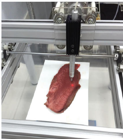
Fig. 2: The device used to control the speed of irradiation
