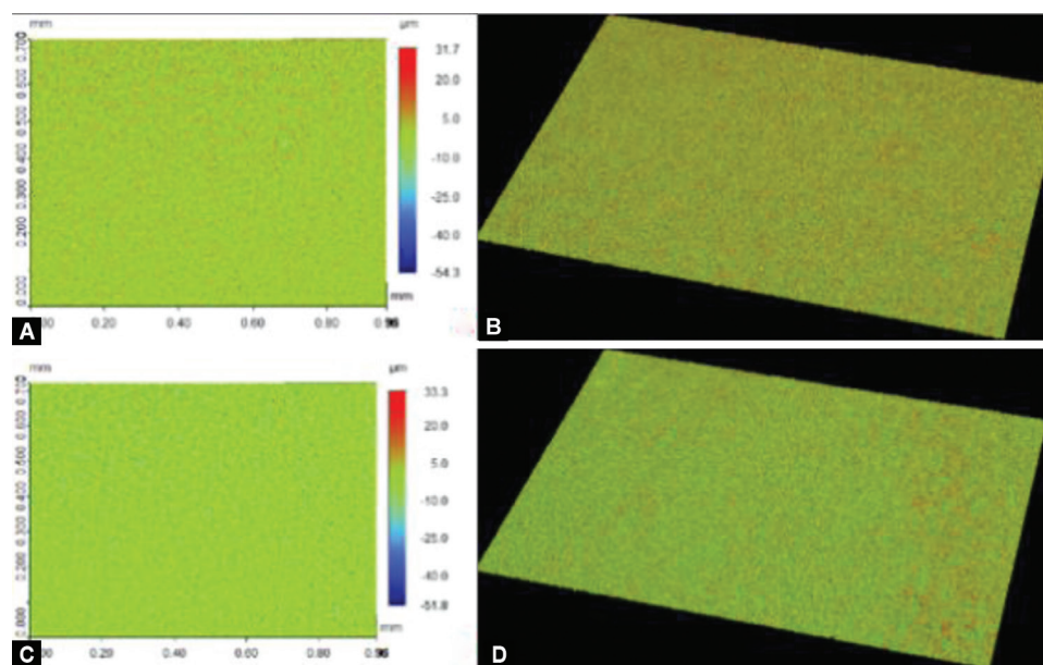
Figs 2A to D: 3D images of the Ra graphical outputs of (A) White LDGC background; (B) Black LDGC background; (C) Zirconia white background; and (D) Zirconia black background
