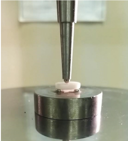
Fig. 1: Specimen setup during biaxial forces strength application
